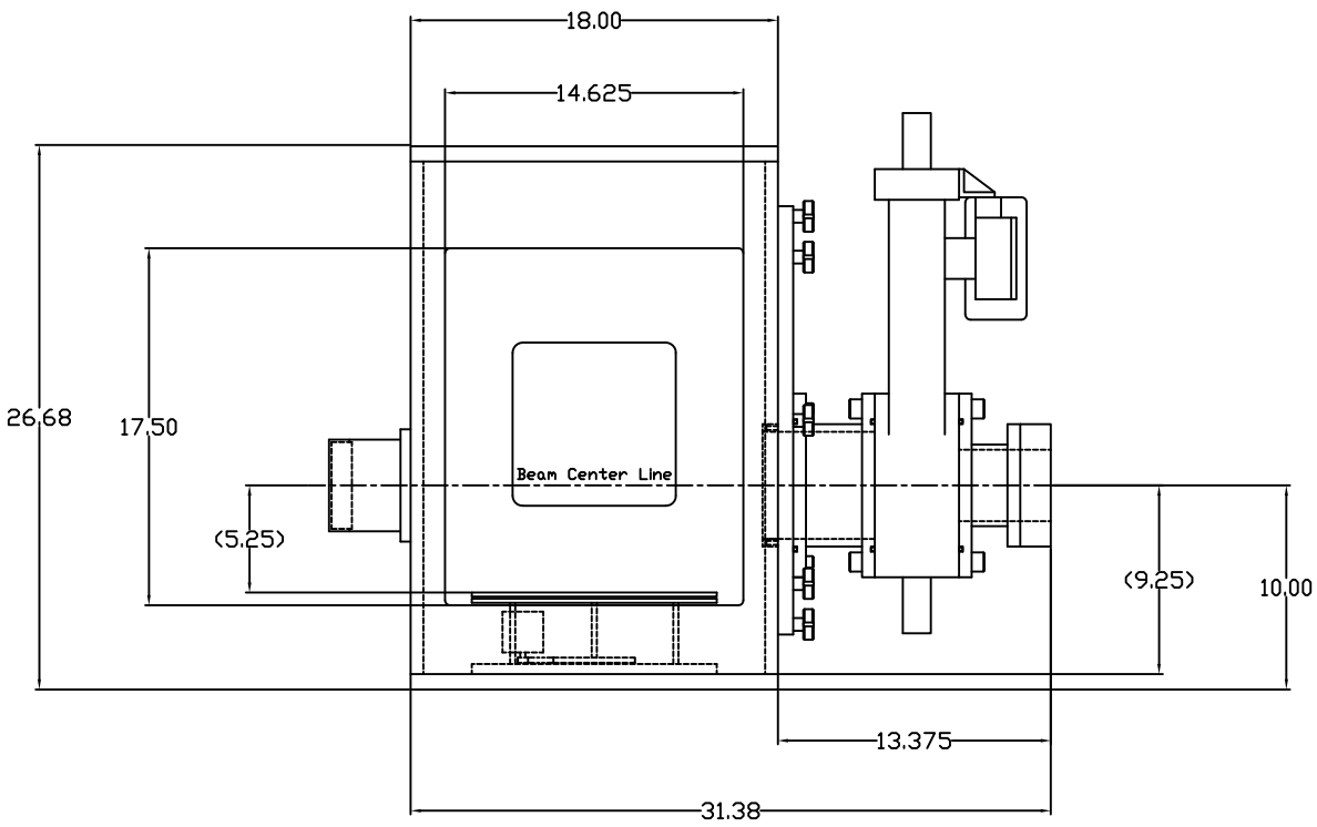
Beam Line #2 Chamber Outline April 2010
